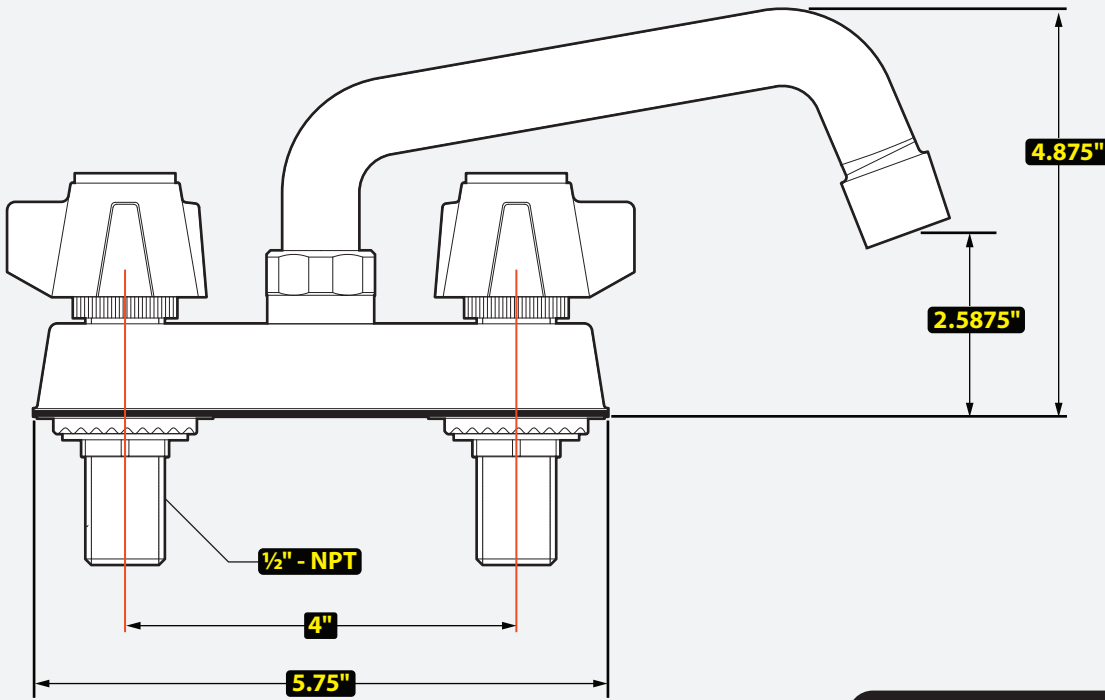
Front View
