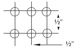
Drain Hole Configuration
